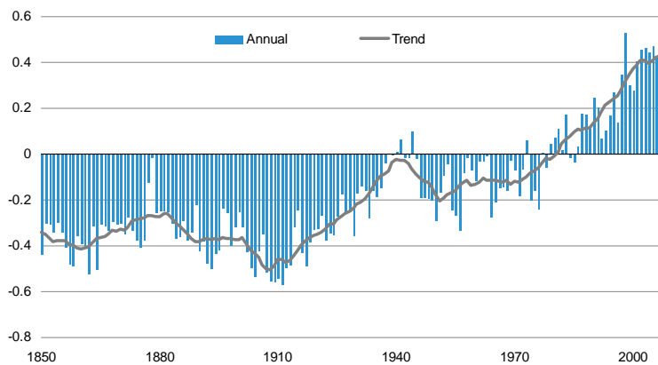
Exhibit 1: The Earth is getting warmer Global temperature deviation relative to average from 1961-1990 in °C
