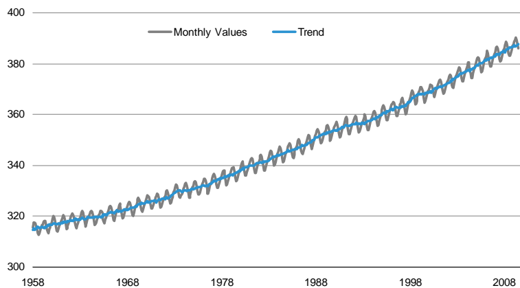
Exhibit 2: CO 2 concentration has been rising CO 2 concentration in Mauna Loa (Hawaii) parts per million
